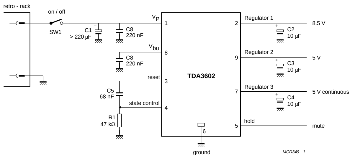
Fig.7 Low end application circuit.
