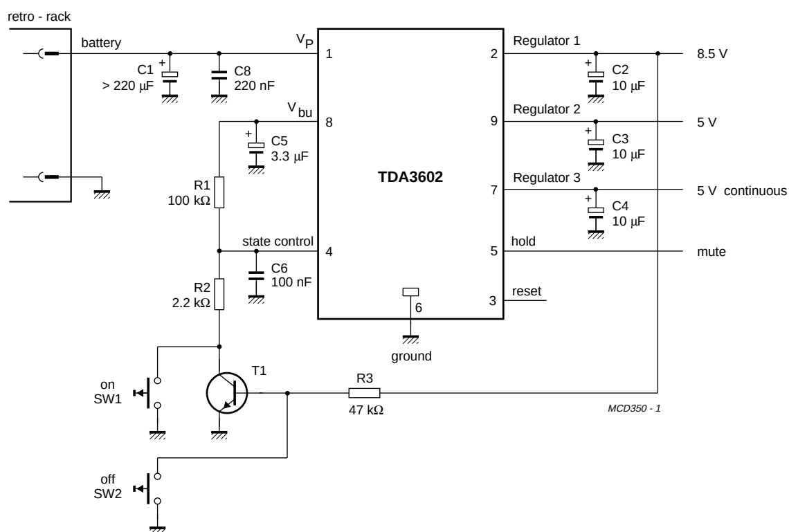
Fig.8 Application circuit 2.
